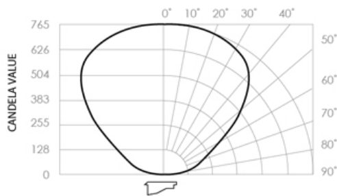
HORIZONTAL CONE at 33°
